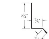
⑨ Drip Cap (DCcc)
