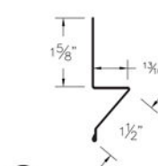
③ Base Angle (BAcc)
