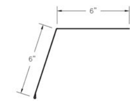
④⑨ Gambrel Trim (GTcc)
