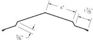
① Universal Ridge Cap (CPcc)
