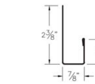
⑥ J Channel (Jcc)
