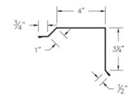
⑤ Gable Flashing (GFcc)
