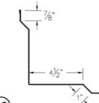
⑬ Inside Corner (ICcc)
