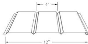
① S 12" Soffit (Solid or Vented)
