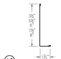
⑩ Post/Fascia Trim (PTcc)
