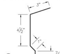
④ Fascia Trim (FTcc)
