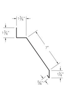
⑮ Face Mount Track Cover (CTcc)
