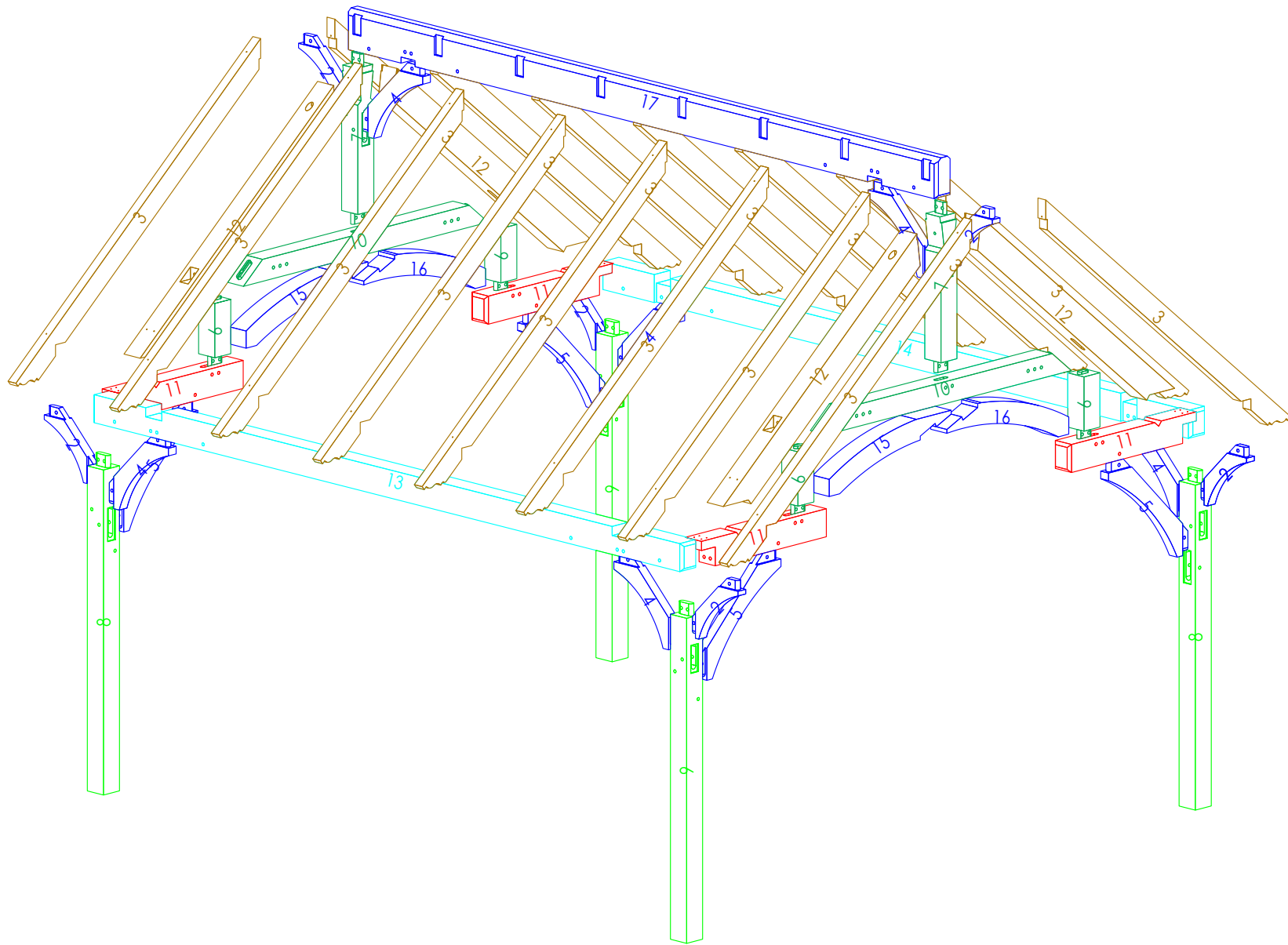
16x18 Grand Teton Timber Frame Pavilion
